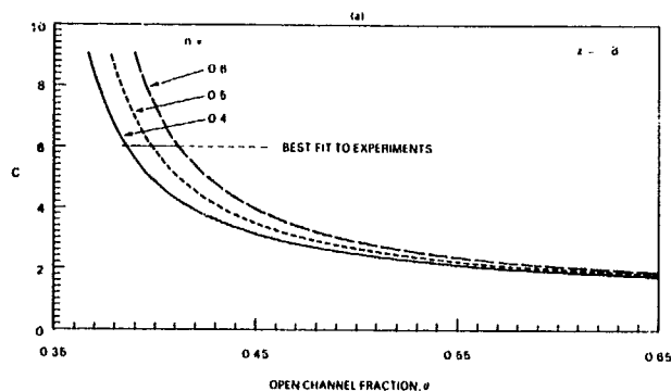
Fig. 14—The coefficient C of the apparent shear rate for the random network with open and closed channels, as a function of \theta and n (a) when z = 8 ; and (b) when z = 4 .
