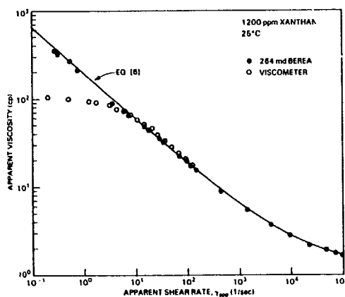
Fig. 3—Comparison of 1,200 ppm xanthan rheology in 264 md Berea sandstone and viscometer at 25°C.
