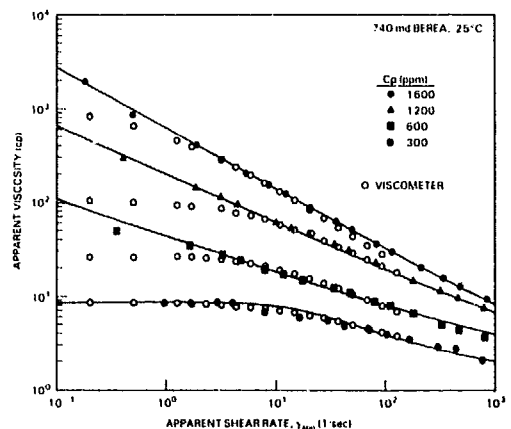
Fig. 8—Comparison of porous media and viscometer rheologies for various xanthan concentrations at 25°C.
