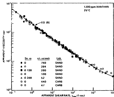
Fig. 7—Summary of flow behavior of 1,200 ppm xanthan in porous media at 25°C.
