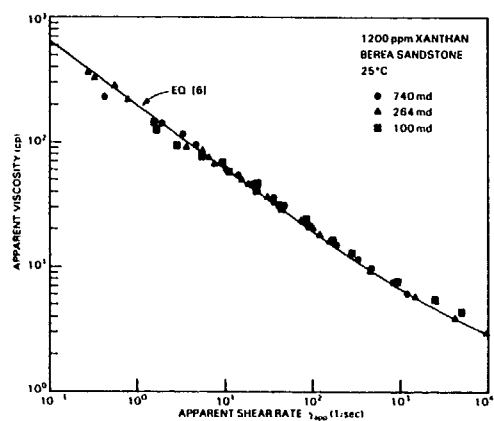
Fig. 4—Influence of Berea sandstone permeability on flow behavior of 1,200 ppm xanthan at 25°C.
