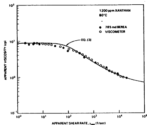
Fig. 9—Comparison of 1,200 ppm xanthan rheology in 765 md Berea sandstone and viscometer at 80°C.
