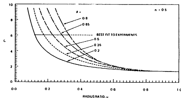
Fig. 13—The coefficient C of the apparent shear rate for the model with z = 2 with a series of constrictions and expansions, as a function of \alpha and \theta when n = 0.5 .
