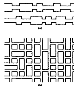
Fig. 12—(a) Capillary bundle model with a series of constrictions and expansions and (b) random network of open and closed channels.
