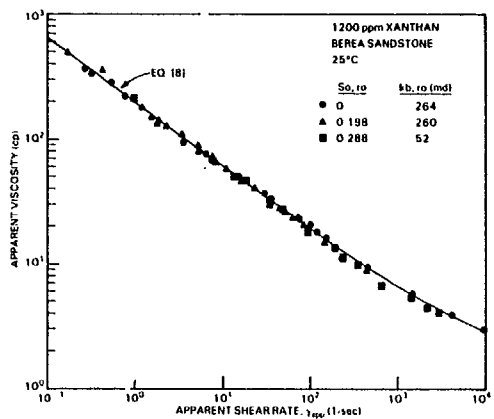
Fig. 6—Influence of residual oil saturation on flow behavior of 1,200 ppm xanthan in Berea sandstone at 25°C.
