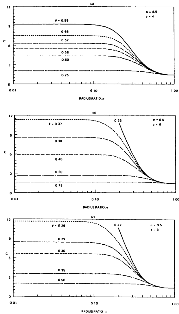
Fig. 15—The coefficient C of the apparent shear rate for the network with bimodal distribution of tube radii, as a function of \alpha and \theta when n = 0.5 and (a) z = 4 ; (b) z = 6 ; and (c) z = 8 .
