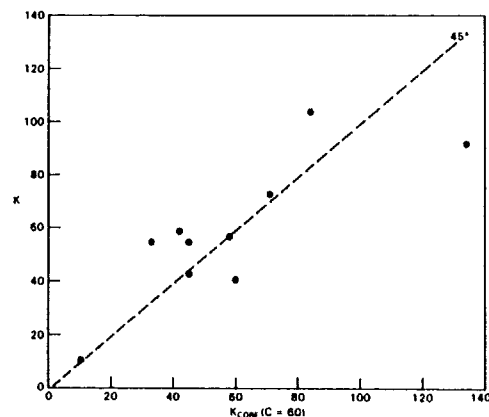
Fig. 10b—Comparison of consistency indices measured in viscometer (K) and calculated from Teeuw and Hesseink's porous media results using value of C = 6.0 obtained in present study ( K_{core} , C = 6.0 ).
