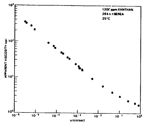
Fig. 2—Flow behavior of 1,200 ppm xanthan in 264 md Berea sandstone.
