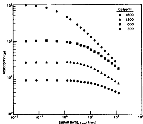
Fig. 1—Viscometer rheology of xanthan solutions at 25°C.
