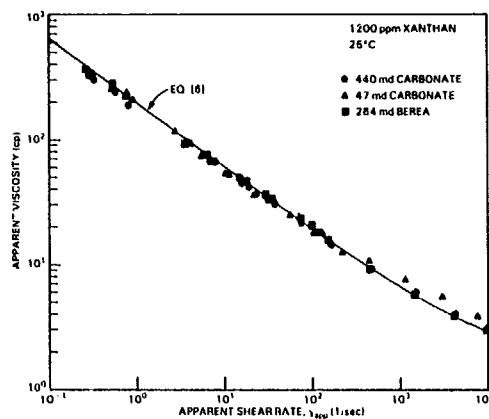
Fig. 5—Influence of lithology on flow behavior of 1,200 ppm xanthan at 25°C.
