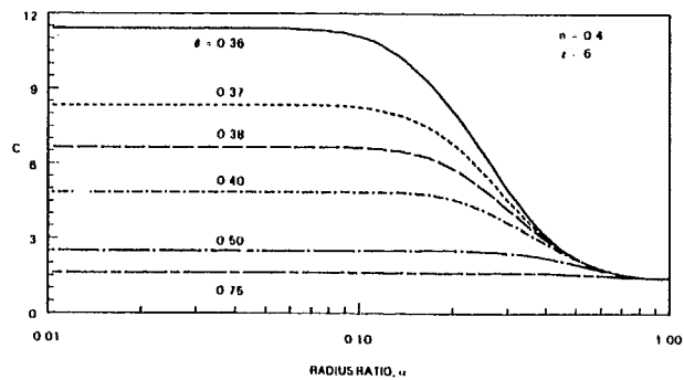
Fig. 16—The coefficient C of the apparent shear rate for the network with bimodal distribution of tube radii, as a function of \alpha and \theta when z = 6 and n = 0.4 .
