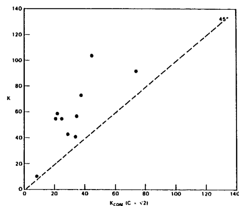
Fig. 10a—Comparison of consistency indices measured in viscometer (K) and calculated from porous media results with C = \sqrt{2} ( K_{core} , C = \sqrt{2} ) by Teeuw and Hesseink (Ref. 1).
